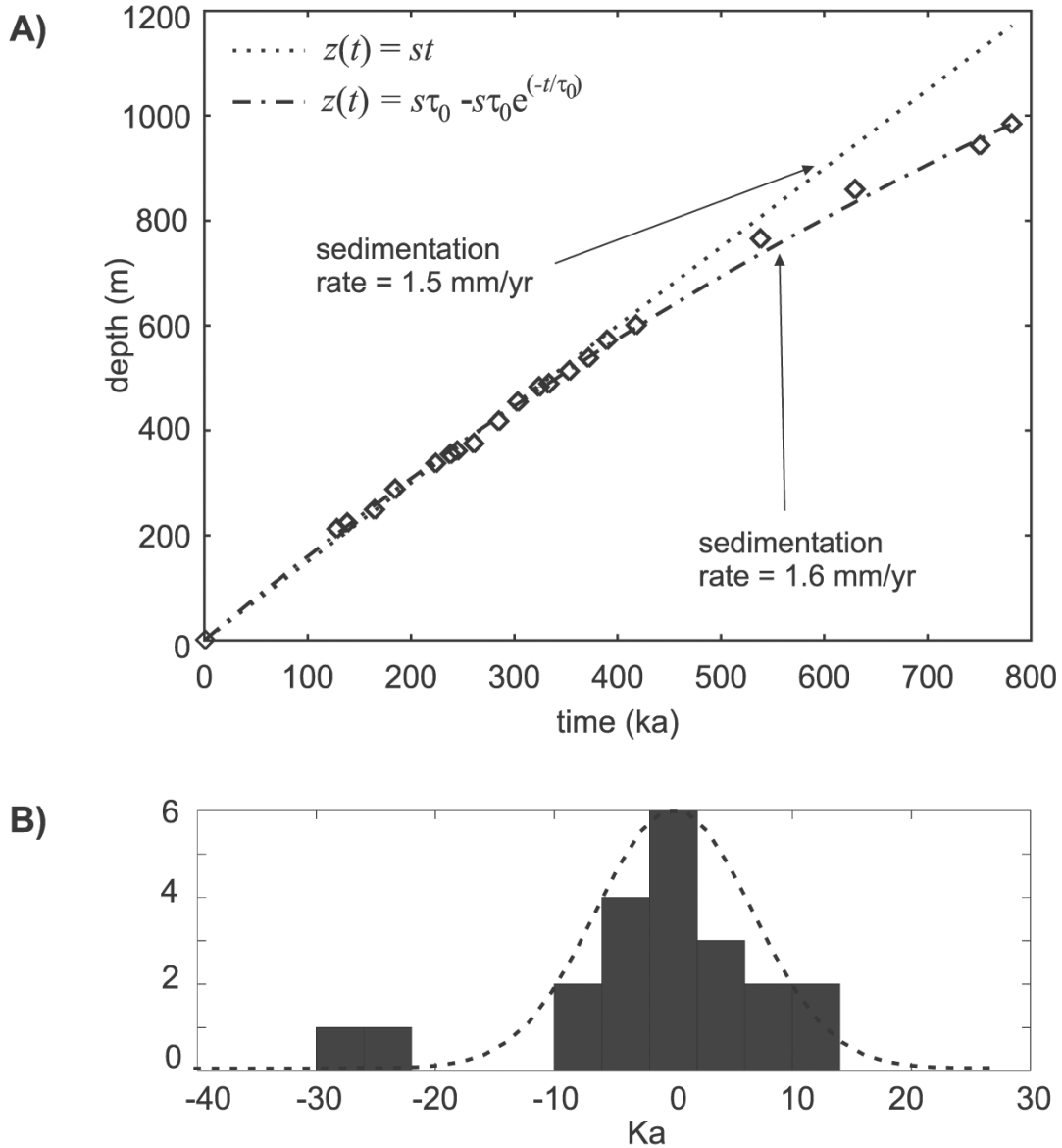
Fig. 4. (A) Time-depth conversion models for ELS1 site. Ages of tie-points in Figure 3 are shown as diamonds. The width of diamonds is twice the uncertainty of ages ( \sim 10 kyr) of tie points. Dotted line corresponds to the linear model z(t)=1.5\text{mm/yr } t , whereas dashed line corresponds to the exponential model z(t)=s\tau_0 - s\tau_0 \exp(-t/\tau_0) , where s=1.6 mm/yr and \tau_0=1530 kyr. (B) Histogram showing the distribution of the residuals of the exponential model and a Gaussian distribution model with a standard deviation of \sim 9.7 kyr.
