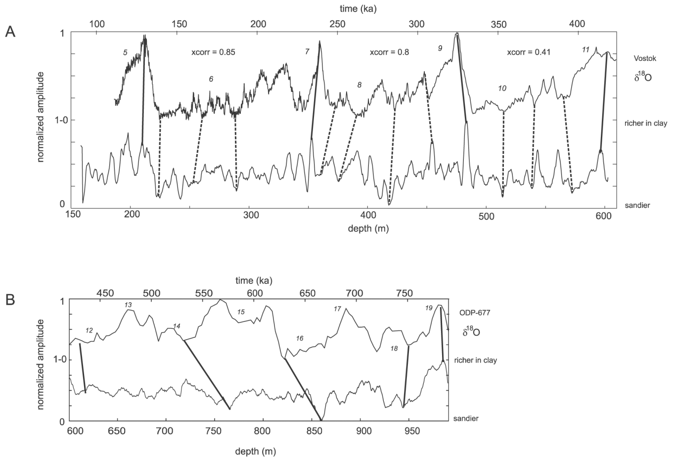
Fig. 3. Correlation between the ELS1 gamma-ray log and \delta^{18}\text{O} signal from Vostok ice cores (A) and \delta^{18}\text{O} from ODP 677 site (B). Vertical scale of both signals has been normalized. Gamma-ray log has been smoothed with a running average of 5 data points (1.2 m) for (A) and 9 data points (2 m) for (B).
