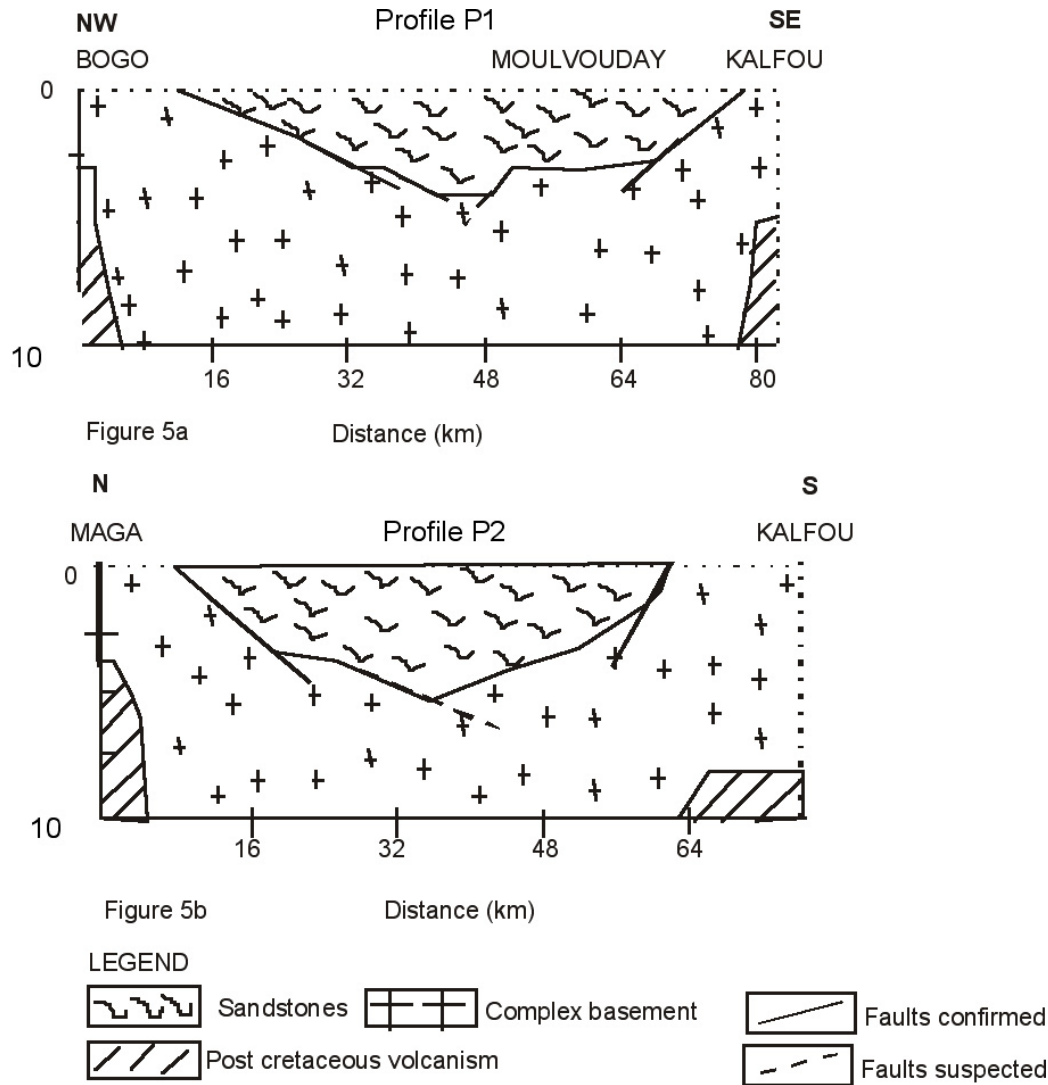
Fig. 5. Geological section of profiles
