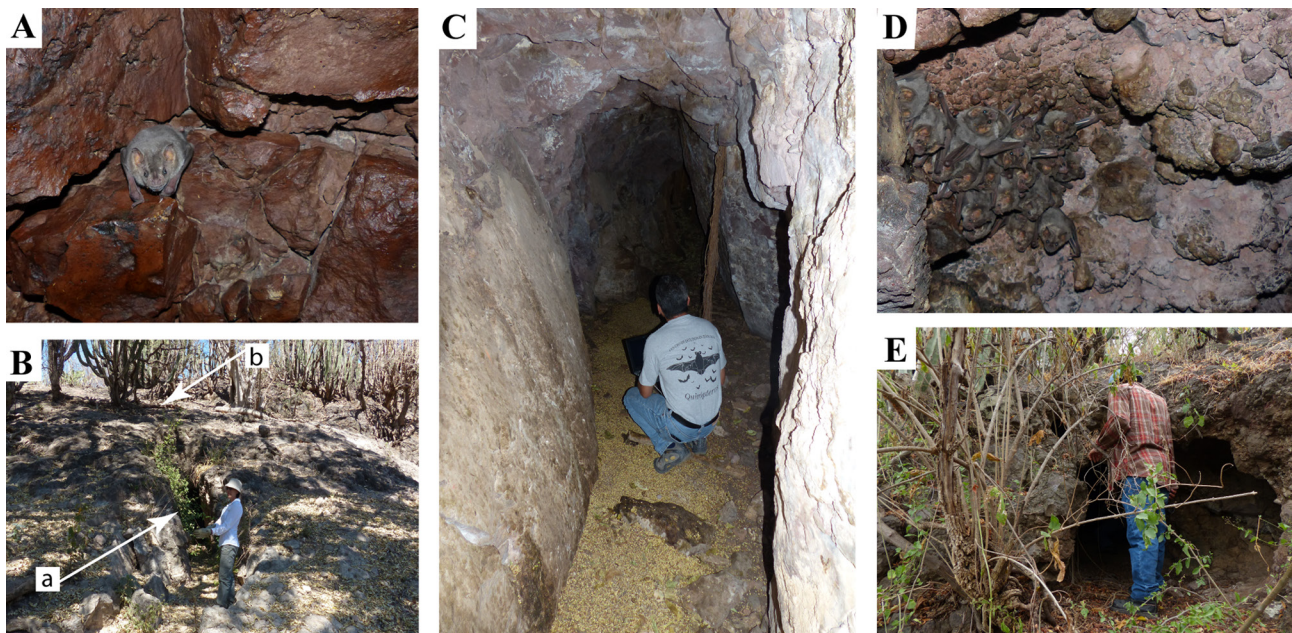
Figure 2. A) Cave 1, crack-with-protrusion roof, and individual of Artibeus hirsutus ; B) cave 1: a) floor-level entrance and b) roof-level entrance; C) cave 1 interior; D) cave 2, crack-with-protrusion roof, and harem of Artibeus hirsutus ; E) cave 2 entrance.
