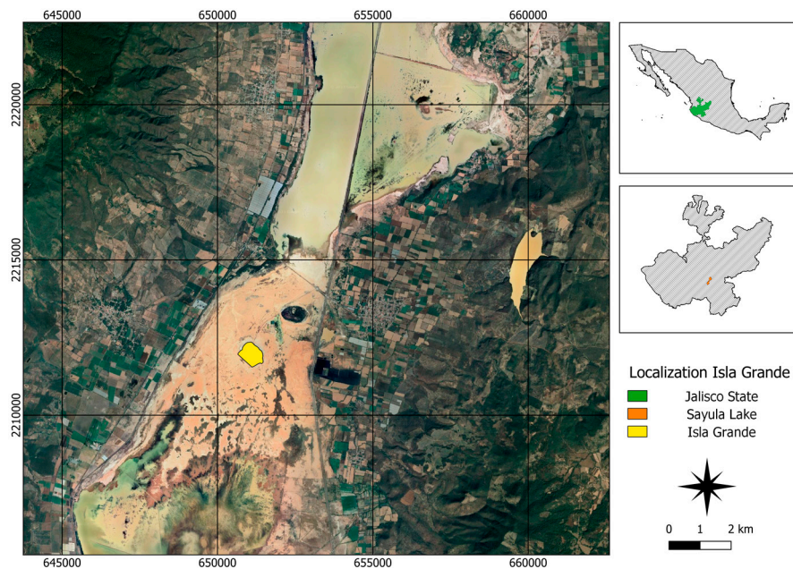
Figure 1. Location of Isla Grande at Lake Sayula, Jalisco, Mexico.
