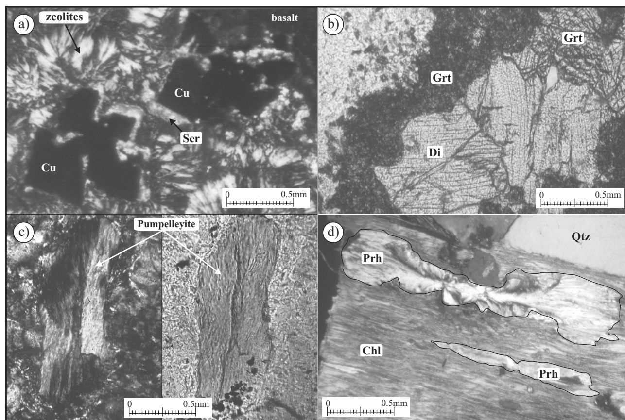
Figure 3. Microphotographies of the most characteristic assemblages. a: Basalt with native cooper, sericite and zeolites found in locality 1; b: diopside and garnet crystals in a metabasite from locality 1; c: twinned crystal of pumpellyite; d: prehnite and chlorite formed by complete alteration of a primary biotite.
