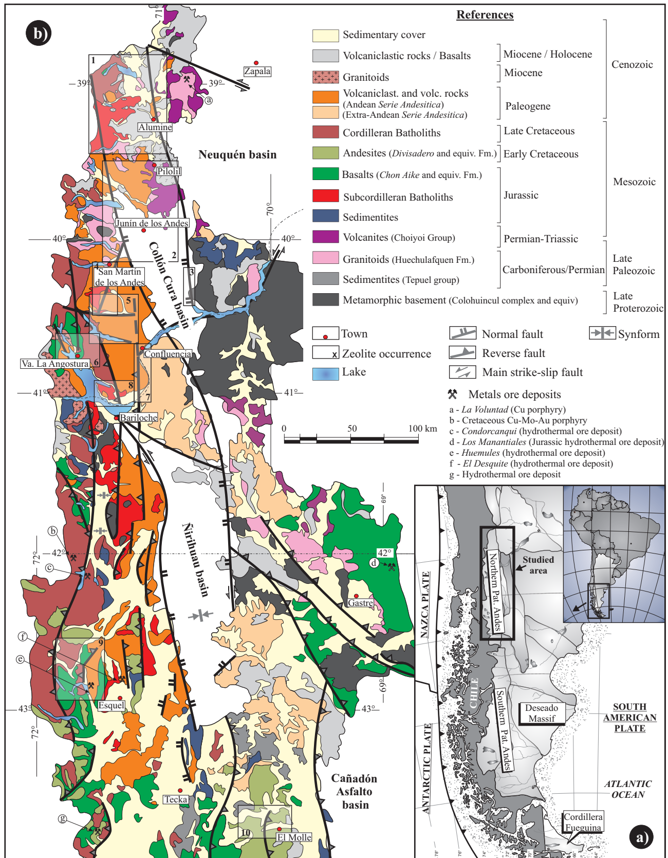
Figure 1. Outline map of the study area showing its different geological units, the major structures and the most important localities where the secondary assemblages described in this paper were sampled (indicated by numbered rectangles); localities are listed in Table 1.
