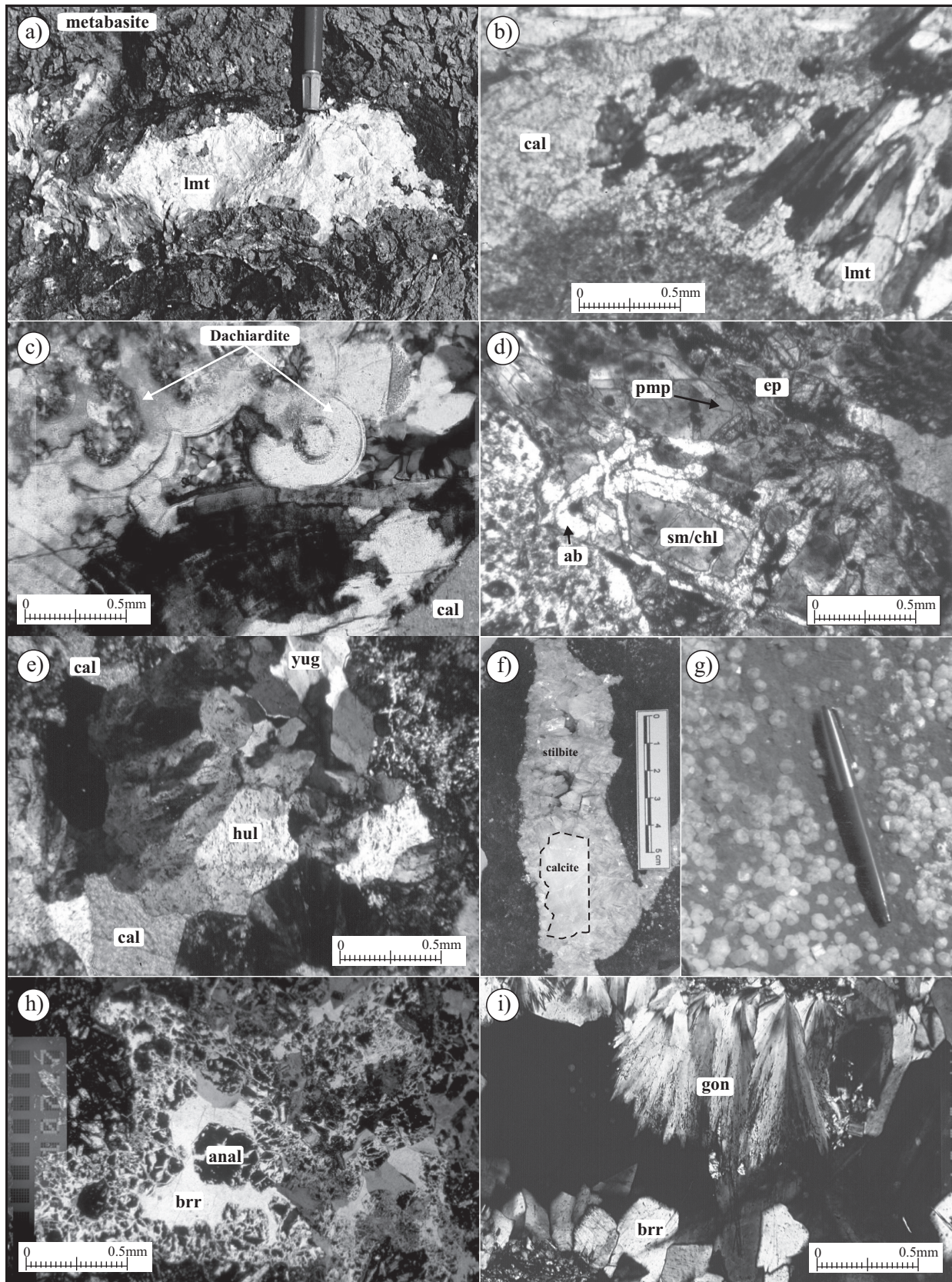
Figure 5. Microphotographies of the most common secondary minerals generated during stages II and III. a, B: Laumontite and calcite assemblages in metavolcanites; c: dachiaridite aggregates; d: albite, epidote, chlorite, smectite and pumpellyite assemblages; e: calcite, heulandite and yugawaralite; f: basalt cavities filled by stilbite and calcite (locality 6); g: small crystals of analcime covering joint planes; h: analcime and barrerite; i: vesicles filled by barrerite and gonardite.
