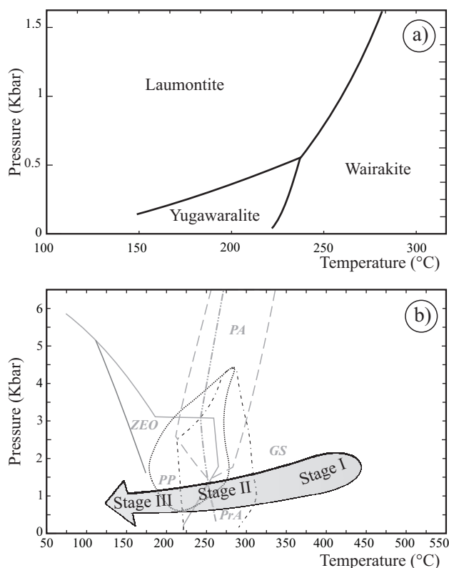
Figure 6. a) P-T diagram showing the stability relationship among yugawaralite, laumontite and wairakite after Zeng and Liou (1982), Liou et al. (1985) and Frey et al. (1991); b) Schematic diagram of the P-T conditions of each stage. P-T fields for low grade metamorphic facies are from Frey et al. (1991); ZEO: zeolites facies, PP: prehnite-pumpellyite facies, PA: pumpellyite-actinolite facies, PrA: prehnite-actinolite facies and GS: greenschist facies.
