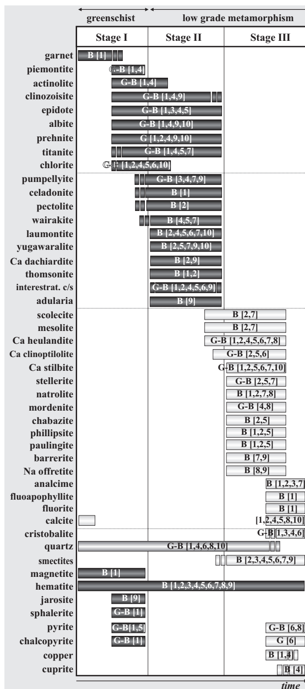
Figure 4. Paragenetic sequence scheme. Wall-rock composition (B=basandesites, G=granitoids) and locality number ([x]) are indicated inside each area.
