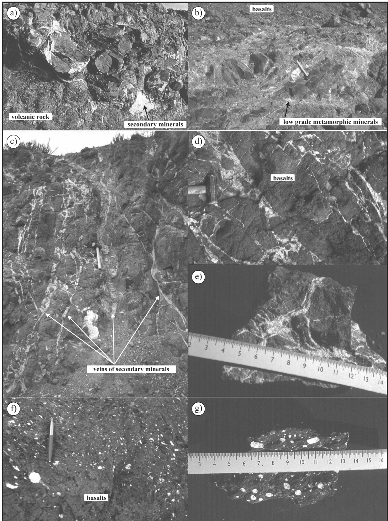
Figure 2. Photographies of the most common secondary textures. a, b: Basalt outcrops from localities 1 and 7 with advanced alteration to low grade minerals; c-e: veins filled with zeolite assemblages, from localities 1 and 10; f, g: vesicles filled with secondary minerals from locality 2.
